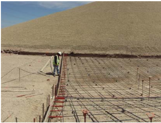
CAMU: South west channel, concrete preparation.
